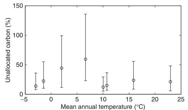
Fig. 12 Relationship between the unallocated carbon, calculated as the sum of the closure terms for gross primary production (GPP), net primary production (NPP), net ecosystem production (NEP), R_e , R_a and R_h and the mean annual temperature. Biomes from left to right: boreal semiarid deciduous, boreal semiarid evergreen, boreal humid evergreen, temperate semiarid evergreen, temperate humid evergreen, temperate humid deciduous, mediterranean warm evergreen, and tropical humid evergreen.
