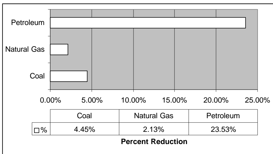
Figure 164: The Effect of an Ideal Location for Biodiesel on Life Cycle Consumption of Primary Energy Resources
